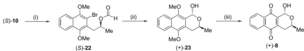
Scheme 5. Reagents and conditions: (i) \text{HCO}_2\text{H} , DCC, 4-DMAP, \text{CH}_2\text{Cl}_2 , 24 h, 0 °C to rt, 85%; (ii) t\text{-BuLi} , THF, 1 h, -78 °C, 76%; (iii) CAN, MeCN– \text{H}_2\text{O} , 10 min, 0 °C, 74%.
