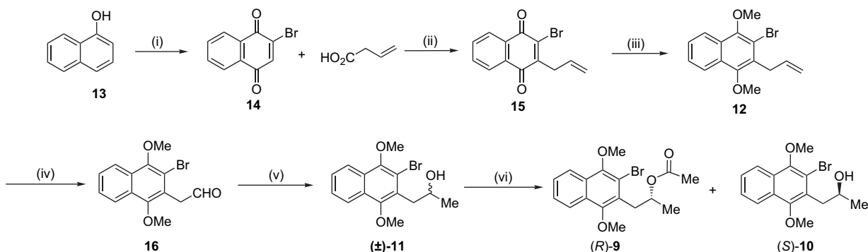
Scheme 2. Reagents and conditions: (i) NBS, AcOH–H 2 O, 1 h, 45 °C, 87%; (ii) AgNO 3 , (NH 4 ) 2 S 2 O 8 , MeCN–H 2 O, 2 h, 60 °C, 67%; (iii) Na 2 S 2 O 4 , THF, TBAI, aqueous KOH, Me 2 SO, 4 h, 95%; (iv) O 3 , Sudan III ® , CH 2 Cl 2 , 15 min, –60 °C, 72%; (v) MeMgI, Et 2 O, 18 h, –78 °C to rt, 60%; (vi) Novozyme 435 ® , p -chlorophenyl acetate, toluene, 60 °C, 70 W, microwave, 6 h, ( S )-alcohol 10 (40%, 93% ee), ( R )-ester 9 (45%, 99% ee).
