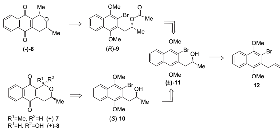
Scheme 1. Retrosynthetic analysis of (–)-9-demethoxyeleutherin 6 , (+)-9-demethoxyeleutherin 7 and 7,9-deoxythysanone 8 .
