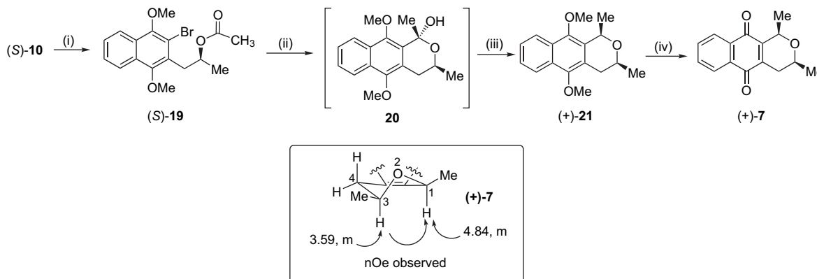
Scheme 4. Reagents and conditions: (i) Ac 2 O, CH 2 Cl 2 , HClO 4 , 2 h, rt, 94%; (ii) t -BuLi, THF, 1 h, –78 °C; (iii) Et 3 SiH, CF 3 CO 2 H, 2 h, rt, 82% (over two steps); (iv) CAN, MeCN–H 2 O, 10 min, rt, 72%.
