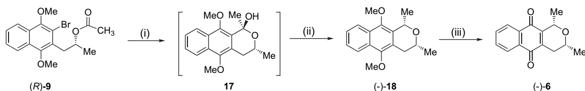
Scheme 3. Reagents and conditions: (i) t -BuLi, THF, 2 h, –78 °C to rt; (ii) Et 3 SiH, CF 3 CO 2 H, CH 2 Cl 2 , 2 h, –78 °C to rt, 70% (over two steps); (iii) CAN, MeCN–H 2 O, 10 min, rt, 75%, 99% ee.
